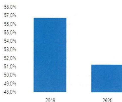
■ Quick Ratio
