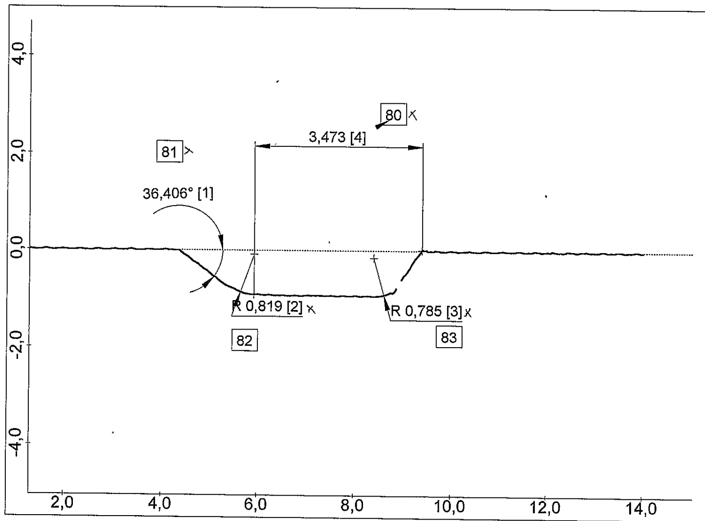
PERTHOMETER CONCEPT
